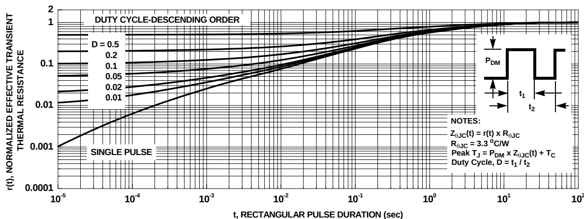
Figure 16. Junction-to-Case Transient Thermal Response Curve for FDPF2D3N10C
